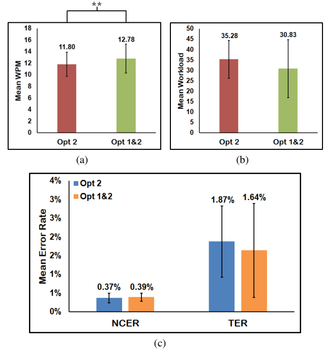
Fig. 8: The comparisons of mean typing speed (a), workload (b), and error rates (c) of the flower keyboard (with QWERTY letter layout) between with all options and without colored keys. Error bars indicate standard deviation. Asterisks denote statistical significance.
