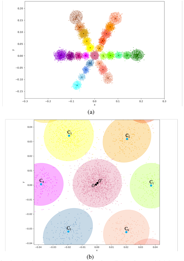
Fig. 9: (a) The scatter plot that contains click-points and 95% confidence ellipses for each key. (b) The central part of (a).
