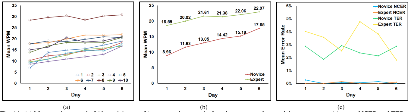
Fig. 11: (a) Mean typing speed of 10 participants, (b) mean typing speed of novice group and potential expert group of 6 sessions, (c) mean NCER and TER of novice group and potential expert group of 6 sessions.
