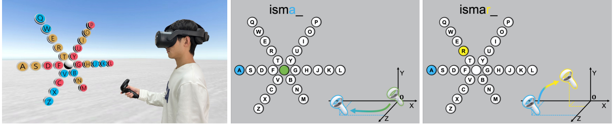
Fig. 1: In the virtual environment, the user holds a controller and applies our Flower Text Entry method to enter text (left). The process of the typing is illustrated in the middle and right images. When the controller is translated from the origin green position to the blue position, the letter ‘a’ is selected for input (middle); then the controller is translated to the yellow position, and the letter ‘r’ is selected for input (right).
