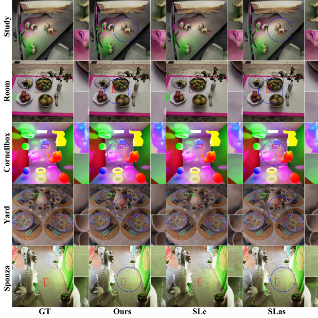
Fig. 4: Comparison between GT (column 1), Ours (column 2), SL_e (column 3) and SL_{as} (column 4) in different scenes. The details in the rectangular regions are magnified and placed on the right of each image.
