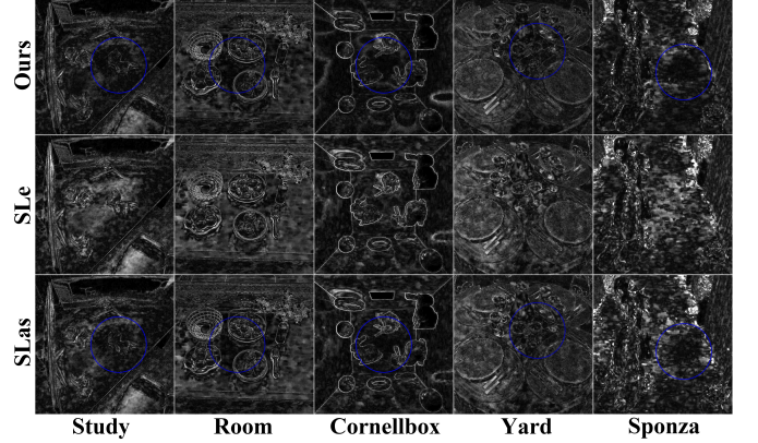
Fig. 5: Visualization of MSE of our method, SL_e and SL_{as} in different scenes. ground truth, MSE_d for the pixels of the diffuse parts in the rendering results compared with the ground truth, MSE_g for the pixels of the glossy parts in the rendering results compared with the ground truth. We measure MSE , MSE_d and MSE_g in the foveal and peripheral regions separately.
