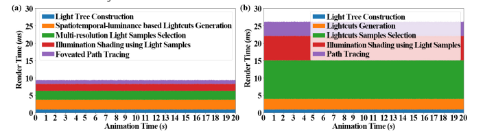
Fig. 9: Time cost in each step of our method (a) compared with that of SL_f (b) in Study .
