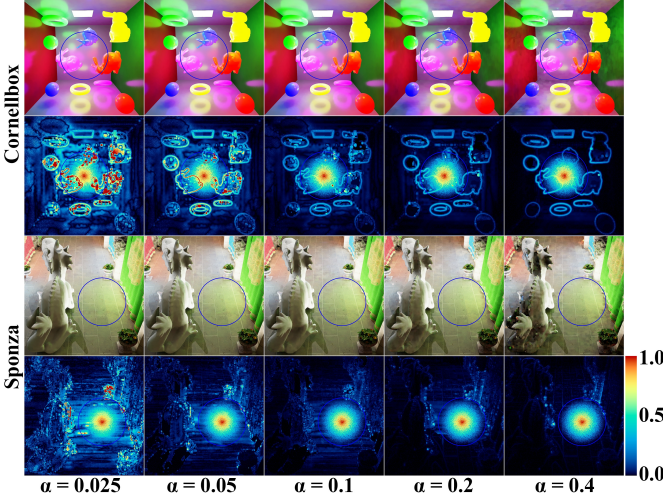
Fig. 7: Rendering results and the FPSM visualization of our method with different values of the maximum imperceptibility threshold \alpha in Cornellbox and Sponza .
