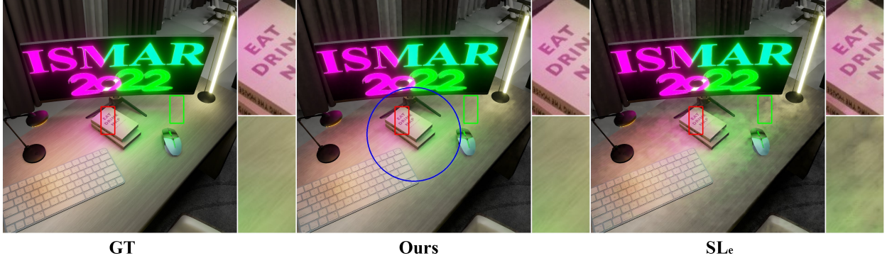
Fig. 1: Many-lights illumination effects rendered by stochastic lightcuts method with 2048 light samples per pixel (left), our method with 5.6 average light samples per pixel (middle), and stochastic lightcuts method using the same rendering time as our method (right) in Study . Compared with stochastic lightcuts ( SL_e ) using the same rendering time as our method, our method achieves 5.3\times smaller mean squared error ( MSE ) in the foveal region ( Ours vs SL_e , 2.47 \times 10^{-2} vs 13.21 \times 10^{-2} ), and 2.3\times smaller MSE in the peripheral region ( Ours vs SL_e , 1.67 \times 10^{-2} vs 3.86 \times 10^{-2} ).
