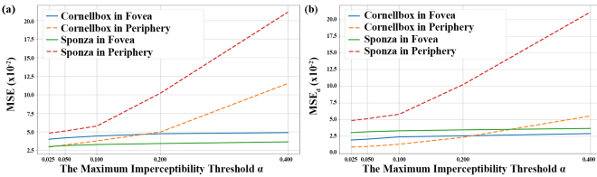
Fig. 8: MSE (a) and MSE_d (b) in Cornellbox and Sponza as a function of the maximum imperceptibility threshold \alpha .
